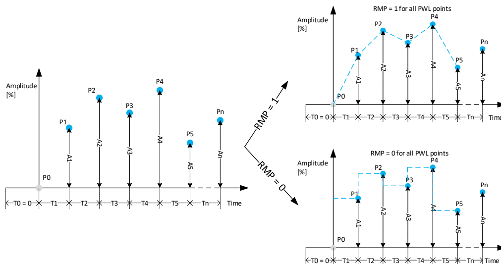
Figure 26: Snippet Example
