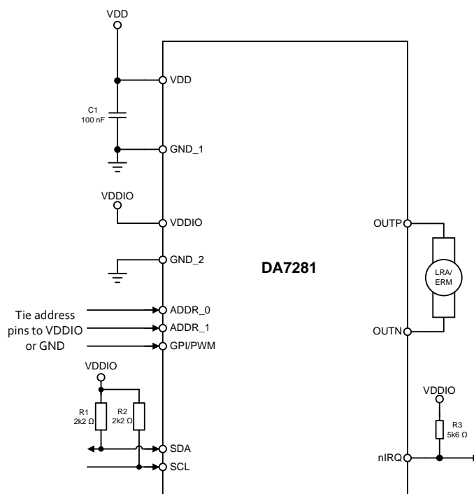
Figure 42: External Components Diagram
