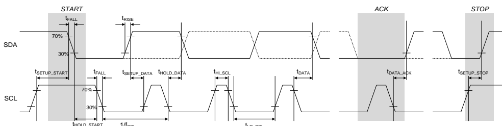
Figure 4: I 2 C Interface Timing
