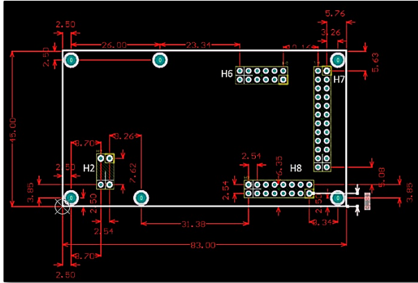
SM2400 EV1Mn-x Top View
