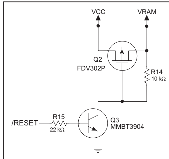
Figure C-3. VRAM Switch
