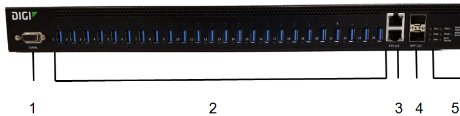
Front panel
