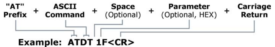
Figure B-11. Syntax for sending AT Commands
