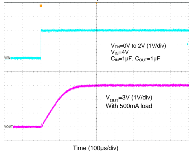
Start-up Time
