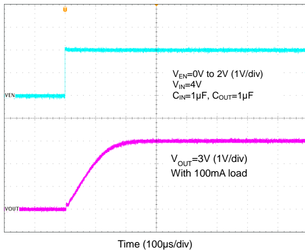
Start-up Time
