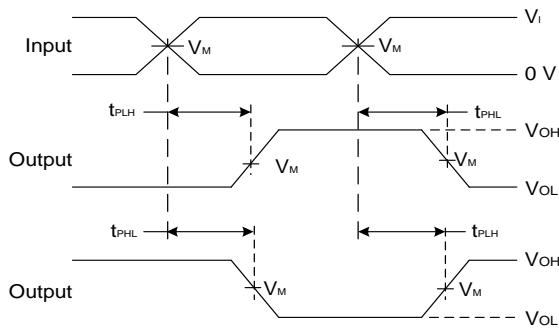
Voltage Waveform Propagation Delay Times Inverting and Non Inverting Outputs (Note 13)
