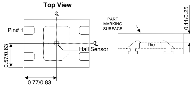
Sensor Location
