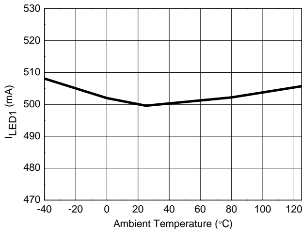
Regulation Current of Channel 1(AL1781) vs. Ambient Temperature Regulation Current of Channel 1(AL1782) vs. Ambient Temperature
