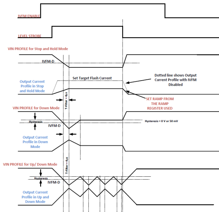
Figure 5. IVFM Modes
