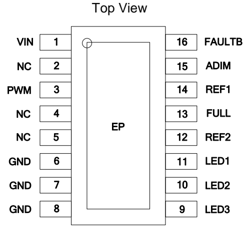
TSSOP-16EP (Type DX)
