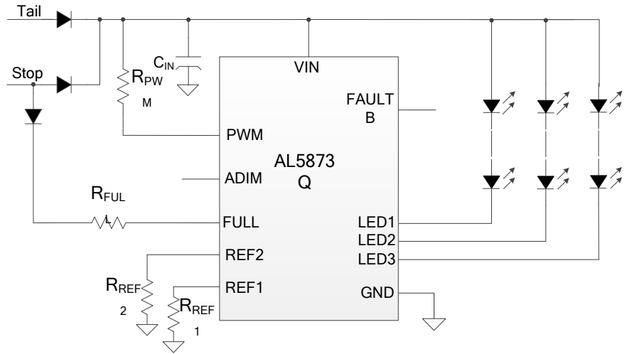
Figure 1. Typical Application
