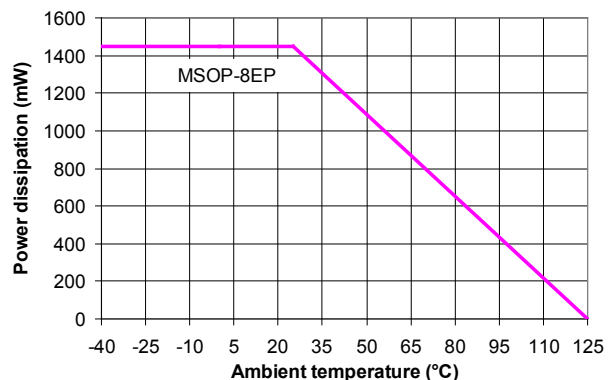
Figure 5 Derating Curve
