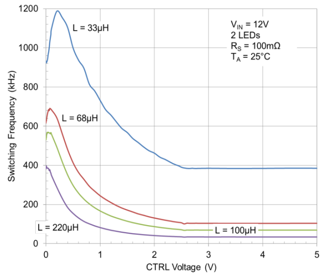
Figure 12 Switching Frequency vs. V_{CTRL}
