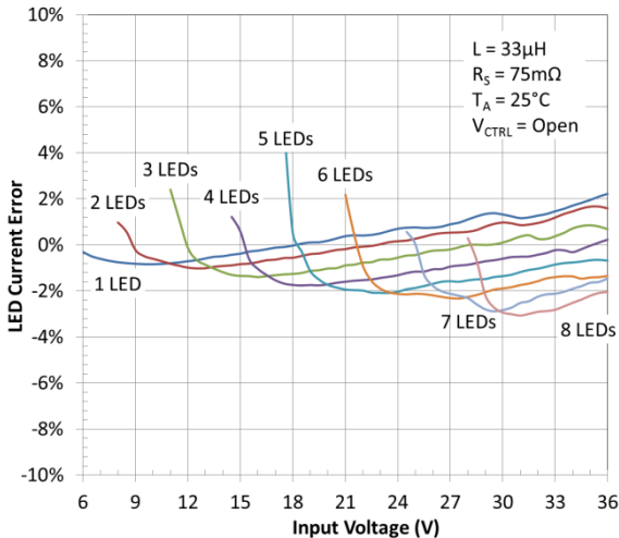
Figure 29. LED Current Deviation vs. Input Voltage
