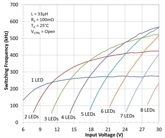
Figure 24. Switching Frequency vs. Input Voltage
