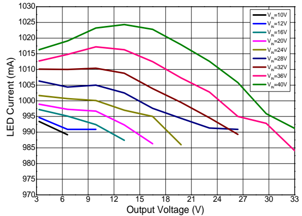
LED Current vs. Output Voltage ( R_{SET} = 0.1\Omega , L = 33\mu\text{H} )
