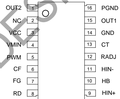
SSOP-16
