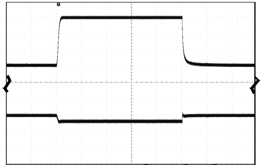
Load Transient ( I_{OUT}=0 to 150mA)
