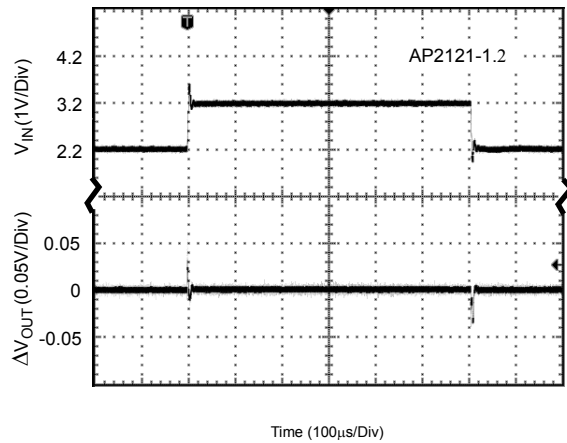
Figure 19. Line Transient (Conditions: I OUT =30mA, C IN =1µF, C OUT =1µF)
