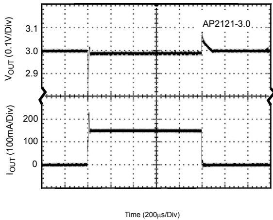
Figure 22. Load Transient (Conditions: V_{IN}=4V , C_{IN}=1\mu F , C_{OUT}=1\mu F )
