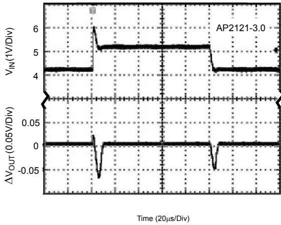
Figure 20. Line Transient (Conditions: I_{OUT}=30mA , C_{IN}=1\mu F , C_{OUT}=1\mu F )
