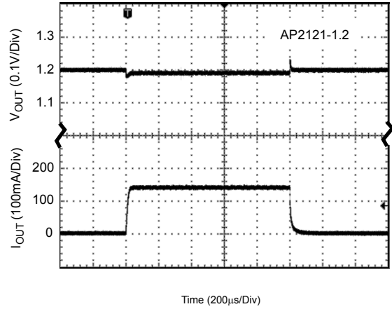
Figure 21. Load Transient (Conditions: V_{IN}=2.2V , C_{IN}=1\mu F , C_{OUT}=1\mu F )
