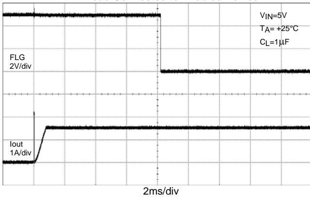
2 \Omega Load Connected to Enabled Device
