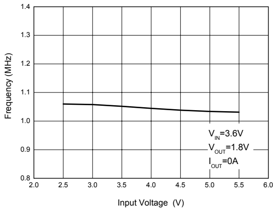
Figure 4. Frequency vs. Input Voltage
