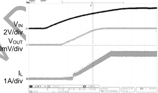
Power on Waveform (V_IN = V_CC = 5V, V_OUT = 1V, I_OUT = 3A)
