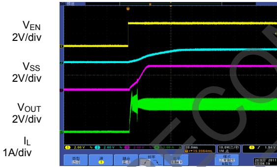
Time 10ms/div
