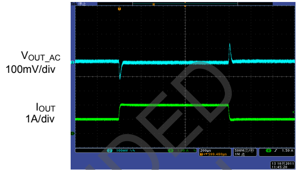
Time 200µs/div
