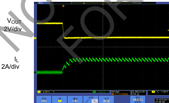
Time 40µs/div
