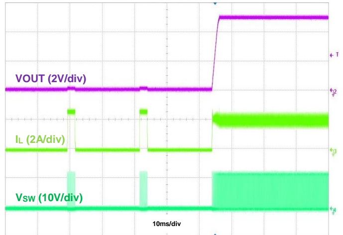
Figure 13. Output Short Recovery, IOUT = 2A
