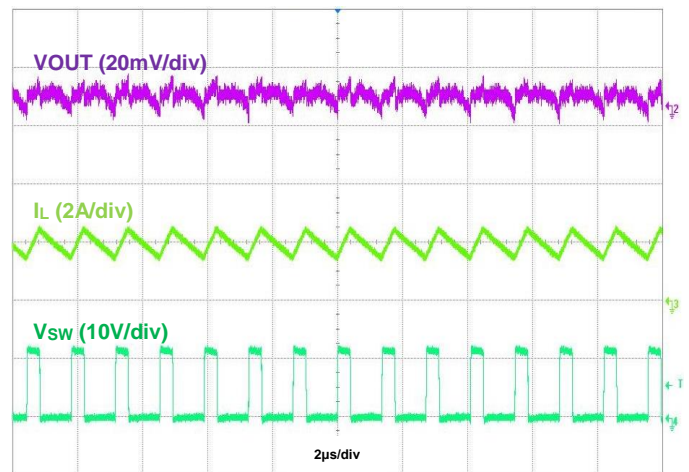
Figure 35. Output Voltage Ripple, V_{OUT} = 3.3\text{V} , I_{OUT} = 2\text{A}
