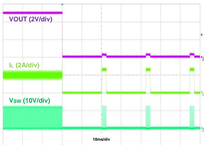
Figure 12. Output Short Protection, I_{OUT} = 2\text{A}
