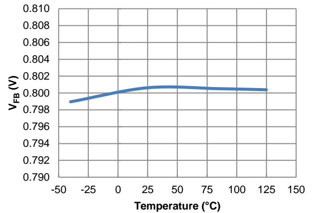
Figure 6. Feedback Voltage vs. Temperature, AP62200/AP62201
