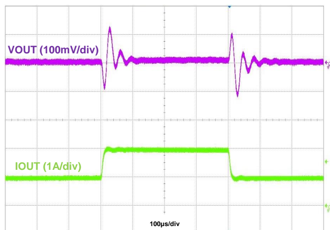
Figure 37. Load Transient, IOU = 1A to 2A to 1A
