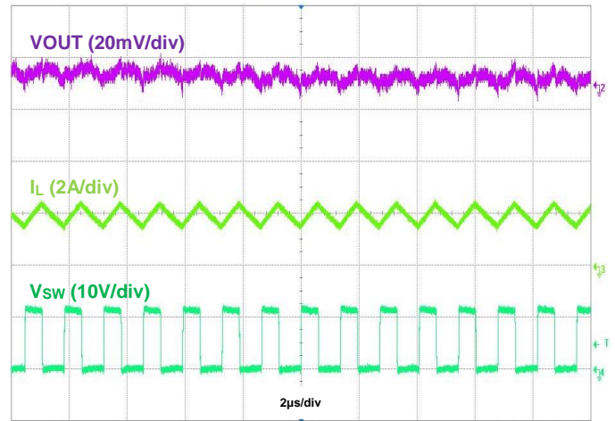
Figure 33. Output Voltage Ripple, V_{OUT} = 5\text{V} , I_{OUT} = 2\text{A}
