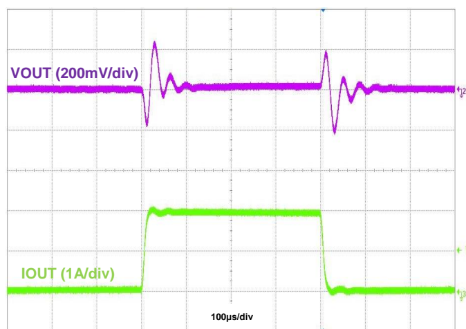
Figure 38. Load Transient, IOU = 50mA to 2A to 50mA
