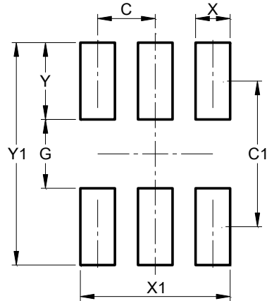
SOT563 (Standard)
