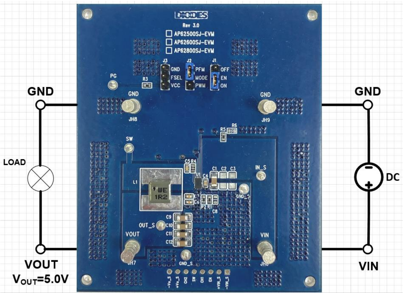
Figure 2. AP62500SJ-EVM
