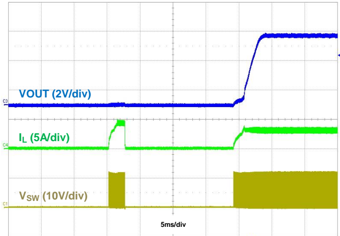
Figure 11. Output Short Recovery, IOUT = 3A
