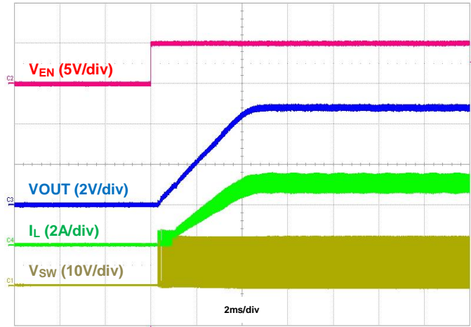
Figure 8. Startup using EN, IOUT = 3A
