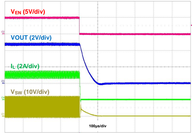
Figure 9. Shutdown using EN, IOUT = 3A
