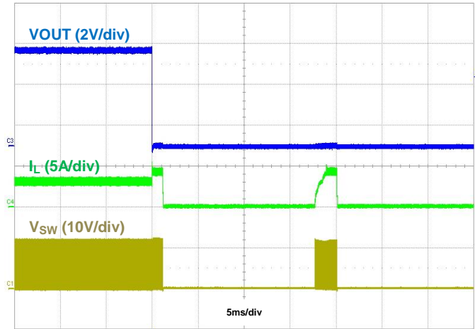
Figure 10. Output Short Protection, IOUT = 3A
