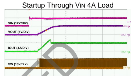
Time-500 \mu\text{s}/\text{div}
