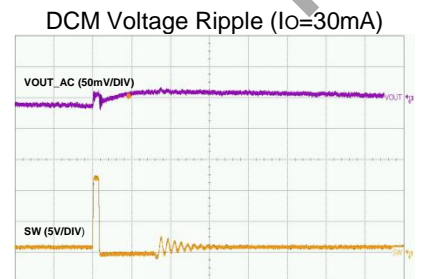
Time-1 \mu\text{s}/\text{div}
