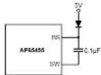
Figure 6 External Bootstrap Diode
