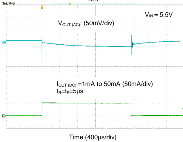
Load Transient Response V_{OUT}=4.5\text{V}
