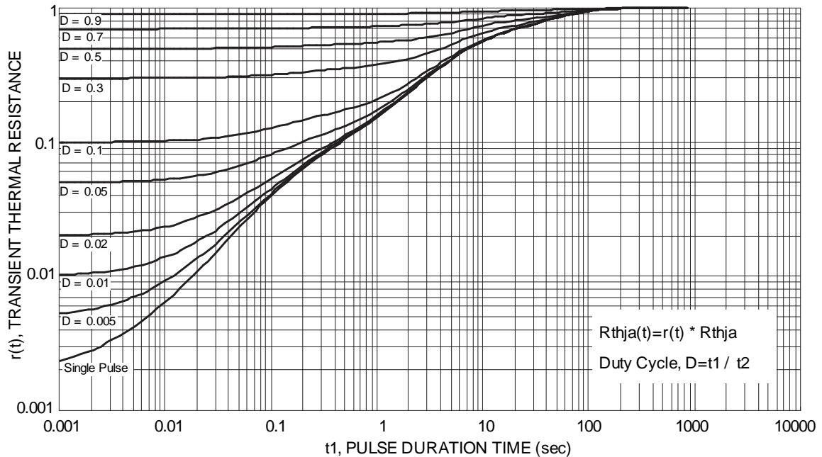
Figure 5 Transient Thermal Resistance
