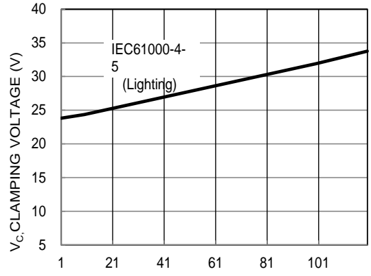
Figure 4 Clamping Voltage Characteristic
