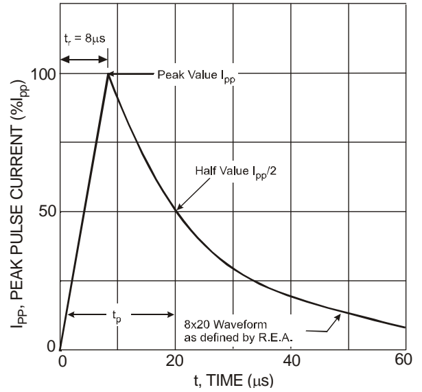
Figure 2 Typical 8 \times 20\mu\text{s} Pulse Waveform
