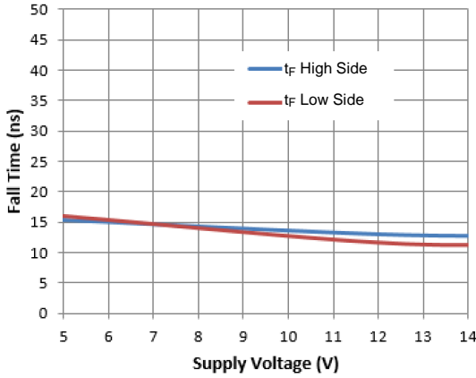
Figure 11. Fall Time vs. Supply Voltage
