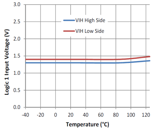
Figure 21. Logic 1 Input Voltage vs. Temperature
