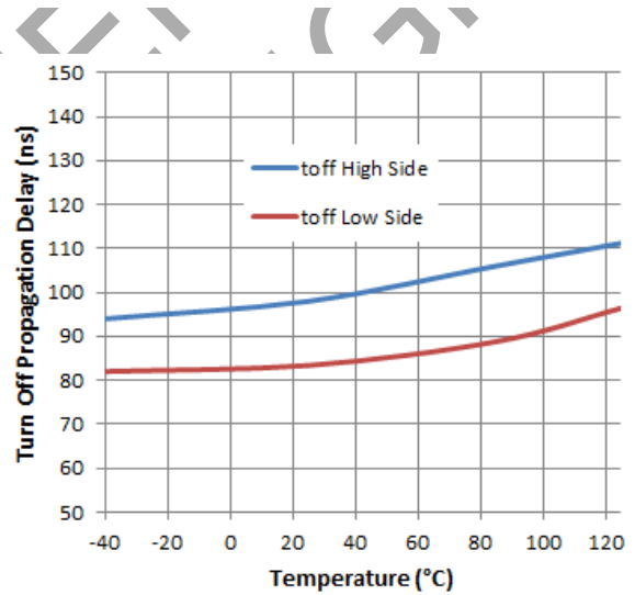
Figure 7. Turn-off Propagation Delay vs. Temperature
