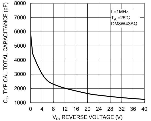
Fig. 6 Typical Total Capacitance (DM8W43AQ Only)
