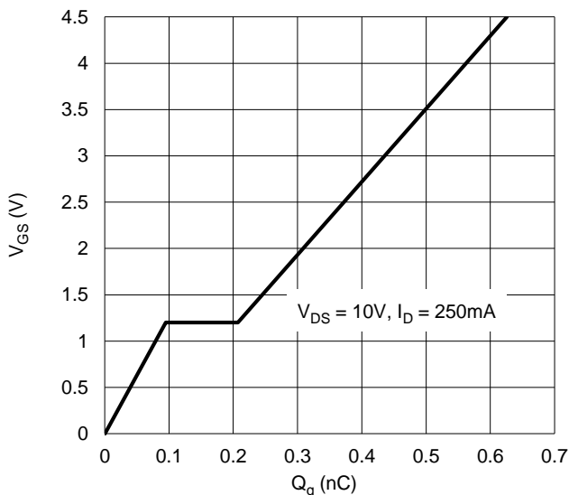
Figure 11. Gate Charge
