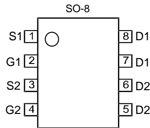
Top View Pin Configuration
