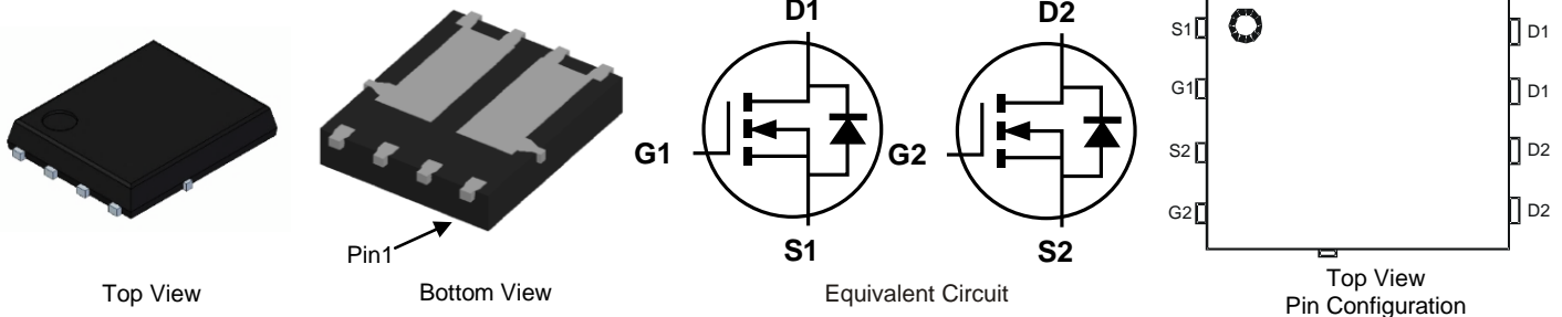
PowerDI5060-8 (Type E)
