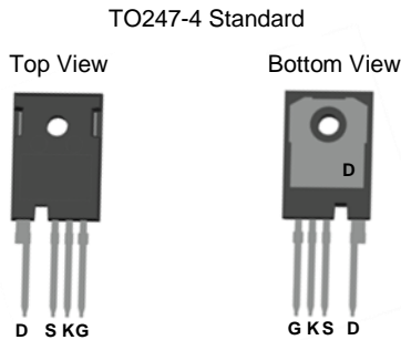
Pin Configuration
