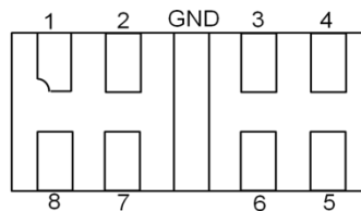
Pin Description (Bottom View)
