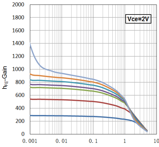
h_{FE} Vs I_c
