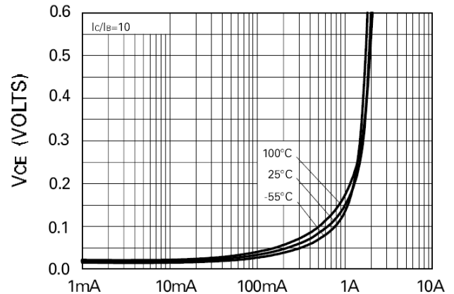
Collector Current V_{CE(SAT)} vs I_C
