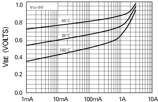
Collector Current V_{BE(ON)} vs I_C
