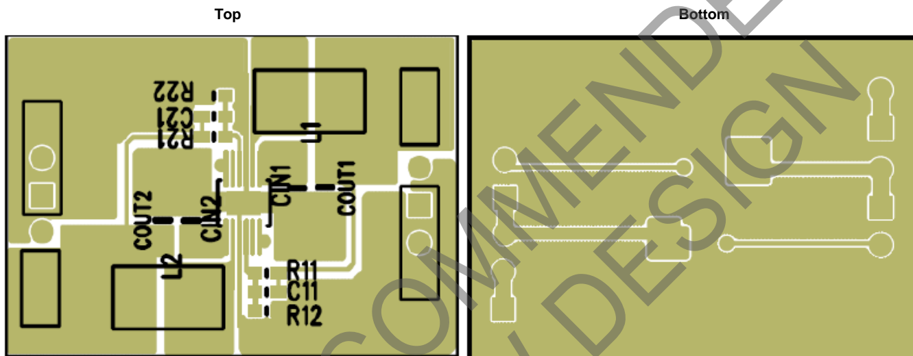
Figure 1. PAM2306D Suggested Layout
