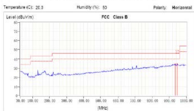
Horizontal Polarization
