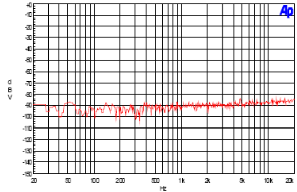
16. Noise Floor
