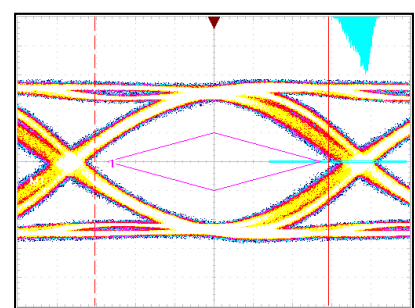
After ReDriver
