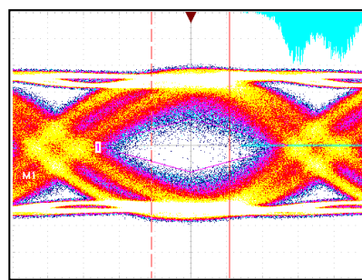
Before ReDriver
