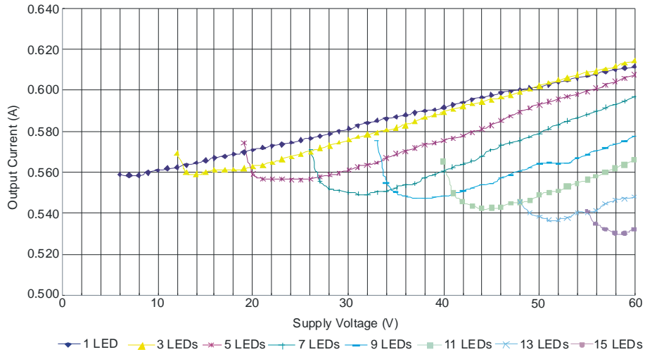
ZXLD1356 Output Current L = 68μH
